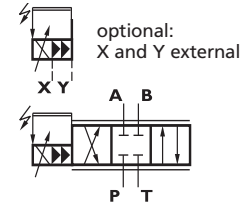
4-way version 3-stage valve
